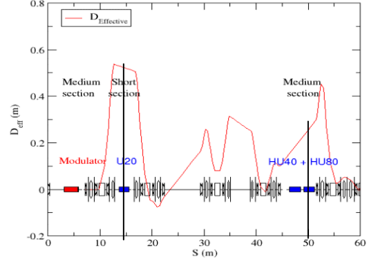
Figure 2: Trajectory of the sliced beam
