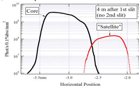
Figure 3: Intensity and separation of the core and the slice
