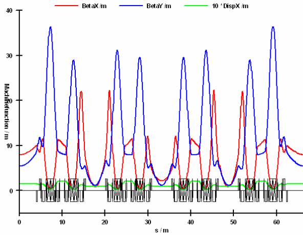
Figure 1 DBA betatron functions for \frac{1}{4} of the ring
