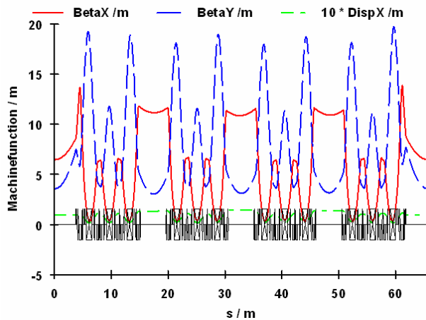
Figure 2 TBA Betatron functions for \frac{1}{4} of the ring
