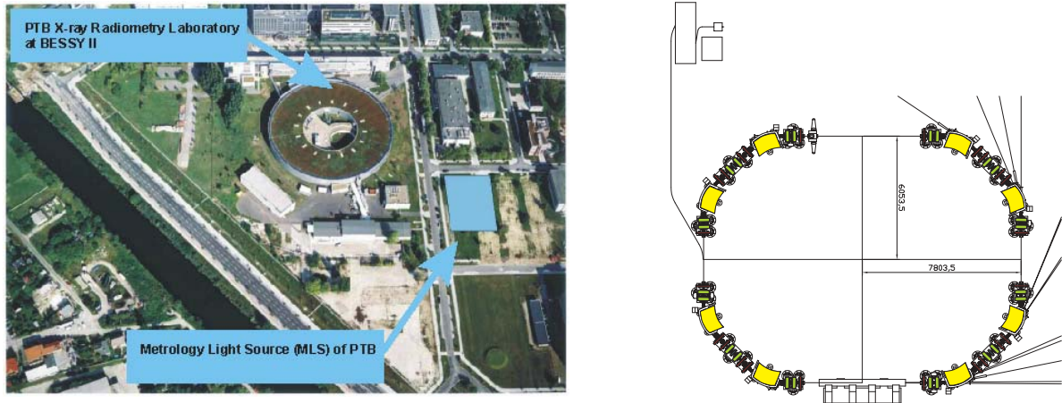
Figure 1: Location (left) and schematic design (right) of the Metrology Light Source (MLS). The MLS is part of the Willv-Wien-Laboratory of PTB constructed in Berlin-Adlershof.
