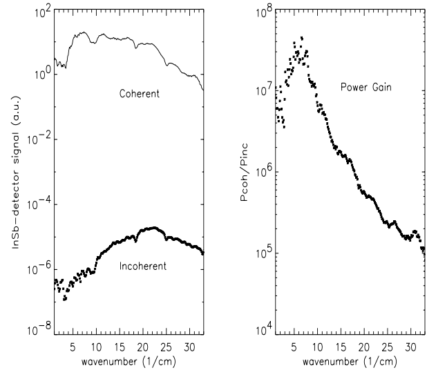
Figure 2: Emitted THz power at 20 mA in the low alpha optics. The left figure part shows raw data of the coherent and incoherent THz power measurements with an InSb-detector. The right figure part shows the ratio of these two intensities, yielding a power gain of more than 10^7 achieved by the coherent emission process.
