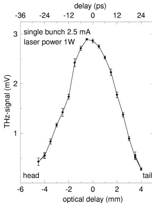
Fig.5 Total THz signal plotted linearly versus optical delay as varied in steps of 500 \mu\text{m} .
