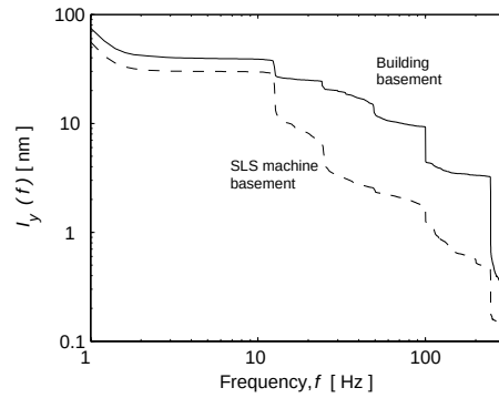
Figure 3: Vertical RMS motion as measured after working hours on the floor of the SLS building (solid line) and on the concrete slab where the SLS machine sits (dashed line).
