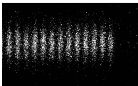
Figure 3. Streak camera view of successive bunches. The full vertical scale is 300 ps and \sigma_{\text{bunch}} = 39 ps.
