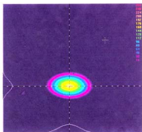
Figure 1. First light observed on the OSR beamline. At the source point \beta_y / \beta_x \approx 25 . Using the theoretical horizontal dispersion and energy spread, the transverse coupling is estimated to be about 1.5%.
