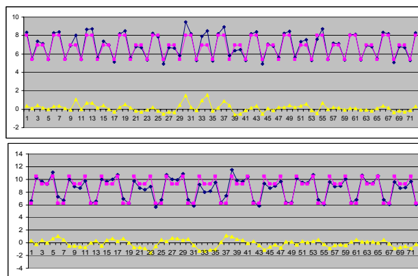
Figure 4. Top: \beta_x at the 72 quadrupoles. Measurements vary from the symmetric model. Lower trace is the difference. Bottom: \beta_y at the quadrupoles (normalized).
