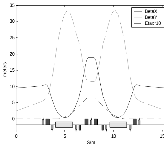
Figure 2: Optical Functions of the Storage Ring Lattice.
