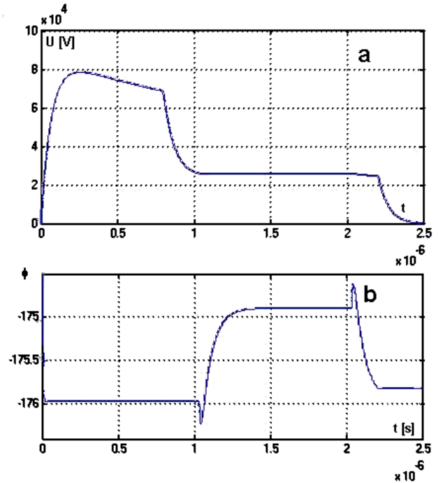
Fig. 3. Amplitude (a) and a phase (b) of the field excited in the Traveling Wave Buncher.
