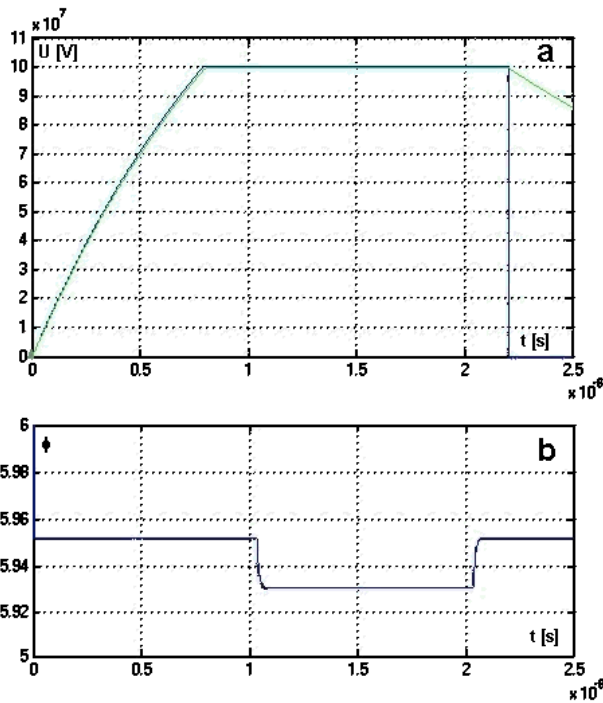
Fig. 4. Field Amplitude (a) and a phase (b) excited in accelerating section.
