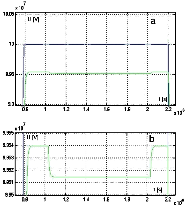
Fig. 5. Change of field amplitude during passage of a beam (magnified 70 (a) and 2000 (b) time)
