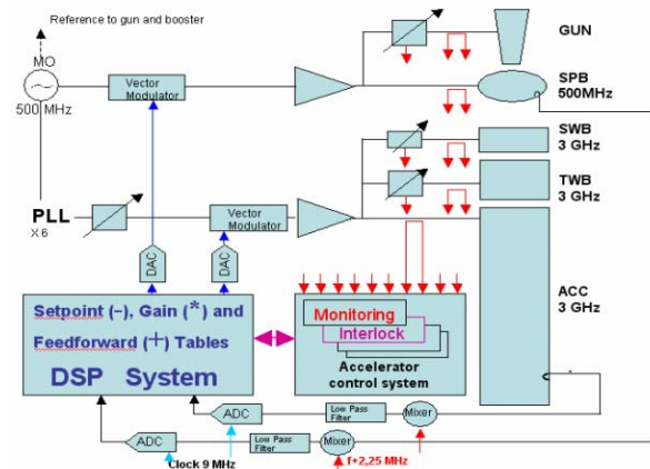
Fig. 1. Scheme of the RF control system for Linac.
