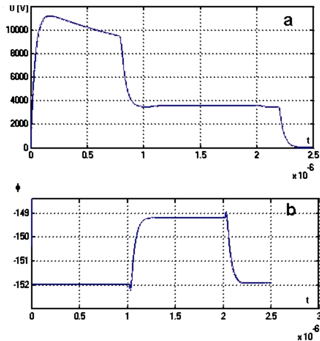
Fig. 2. Amplitude (a) and a phase (b) of the field excited in the Standing Wave Buncher
