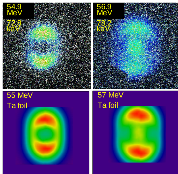
Fig. 5 Radiographs of Ta K-edge.
