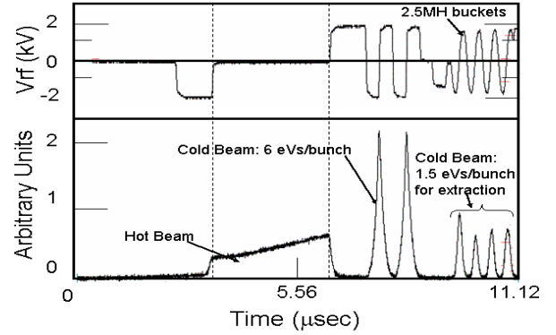
Figure 3: Recycler cavity fanback and wall current monitor signals for anti-proton unstacking for the ppbar collider operation.
