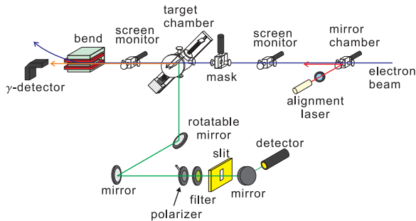
Figure 4: Experimental setup
