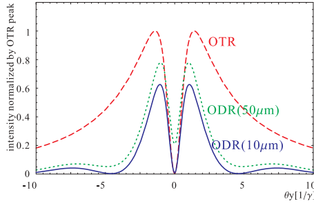
Figure 2: the projected vertical polarization component. solid line is for \sigma_y = 10\mu\text{m} , dotted line is for \sigma_y = 50\mu\text{m} and dashed line is the OTR.
