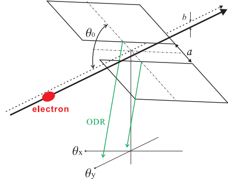
Figure 1: Geometry of ODR from a slit target
