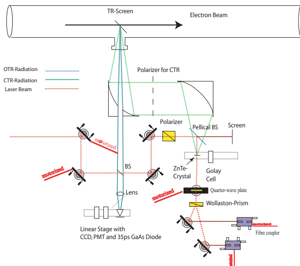
Figure 1: Schematic of the setup inside the linac area.
