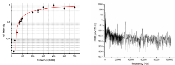
Figure 4: Left: Computed transfer function for CTR radiation from the CTR screen to the ZnTe crystal, convoluted with the laser beam profile at the crystal. The error bars represent the numerical uncertainties. Right: Noise spectrum of the error signal
