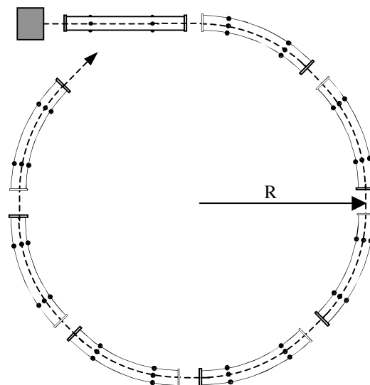
Figure 3. Layout with 7 out of 8 Curved Sections.
