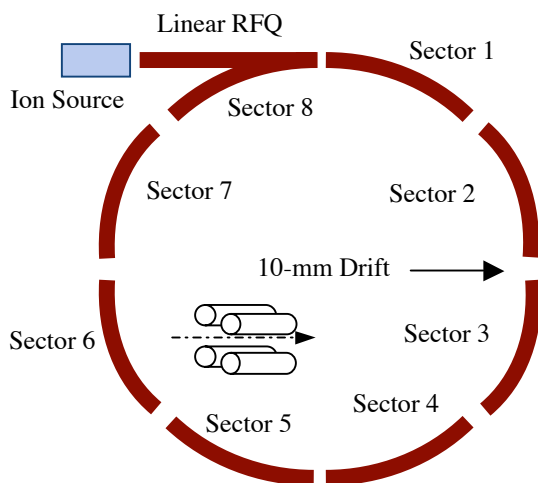
Figure 1. Layout of the CRFQ Prototype in the final stage.
