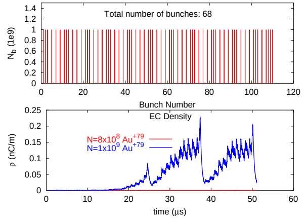
Figure 1: Simulated electron cloud evolution for 68 bunches over 4 turns (lower part). In the upper part the pattern (3,68,52) is shown over one turn. Note that the upper and lower part have different time scales.
