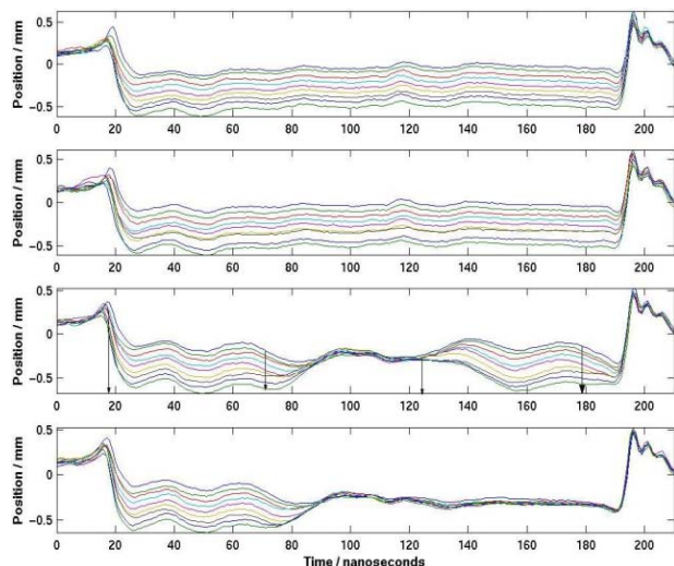
Figure 5: Results from FONT2. Top: beam starting positions. Upper middle: action of the 'beam flattener' to remove slowly-varying components in the bunch position structure within the train. Lower middle: effect of the feedback without delay loop. The arrows show the boundaries between the latency periods during the system operation; 3.2 latency periods are apparent. Bottom: full system including delay-loop feedback.
