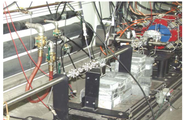
Figure 4: Downstream section of the FONT2 experiment, showing the suite of 3 BPMs. The upstream BPM forms the sensor of the feedback loop; the two downstream BPMs act as independent monitors of the beam position after the correction
