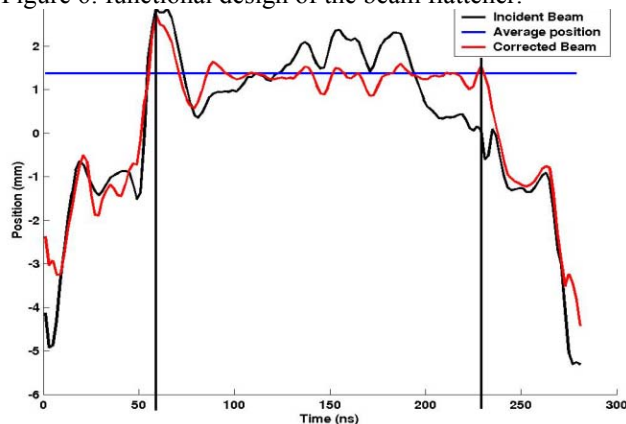
Figure 7: Operation of the beam flattener. The incoming
