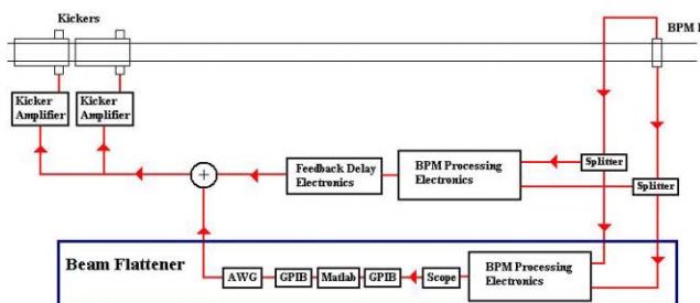
Figure 6: functional design of the beam flattener.
