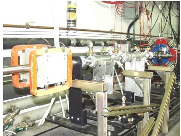
Figure 3: Upstream section of the FONT2 experiment in the NLCTA beamline, showing the dipole magnet for beam steering and the two kickers for beam position correction.
