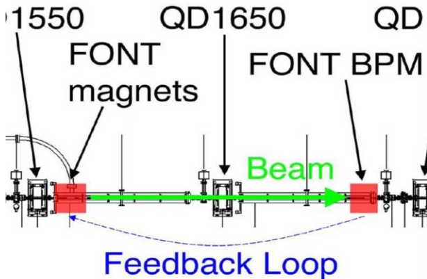
Figure 2: Schematic of the NLCTA beamline showing location of the dipole, kickers and BPMs.
