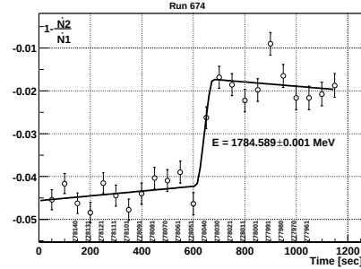
Figure 3: The measurement of the beam energy on a jump in the counting rate of IBS electrons during scanning the frequency of the depolarizer. Energy measured is 1784.589 \pm 0.001 MeV.
