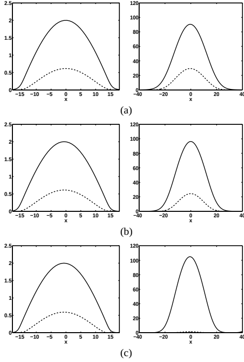
Figure 2: Comparison of soliton solutions with varying \alpha_m = 0.1, 0.5, 0.99 in a low(left side, \lambda = 0.01 ) and a high temperature(right side, \lambda = 30 ). The vector potential a is drawn with solid line and the scalar potential \varphi with dashed line. (a) \alpha_m = 0.1 (b) \alpha_m = 0.5 (c) \alpha_m = 0.99
