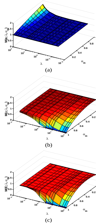
Figure 3: Figure 4. Plot of M(\psi; \lambda, \alpha_m) with \psi = a, \varphi , and E with respect to \alpha_m . The direction of \lambda axis is inverted to show the changes explicitly in (b) and (c). (a) M(a; \lambda, \alpha_m) (b) M(\varphi; \lambda, \alpha_m) (c) M(E; \lambda, \alpha_m)
