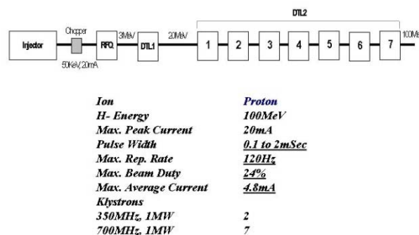
Figure 1: Accelerator structure and parameters of KOMAC
