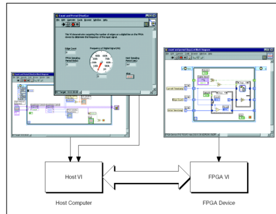
Fig.3 Communication architecture between host and FPGA devices
