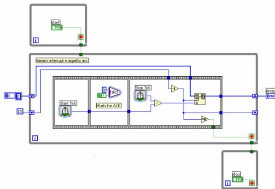
Fig.4 FPGA LabVIEW code to measure communication performances
