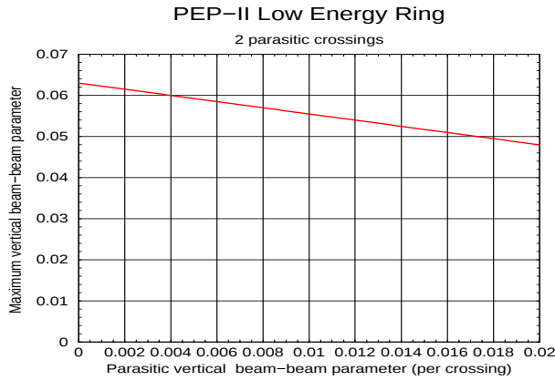
Figure 3: PEP-II Low Energy Ring (2 parasitic crossings): maximum vertical beam-beam parameter, \xi_{y,Max} , with the presence of parasitic crossings vs the parasitic crossing vertical beam-beam parameter per crossing, \xi_{PC,y} .
