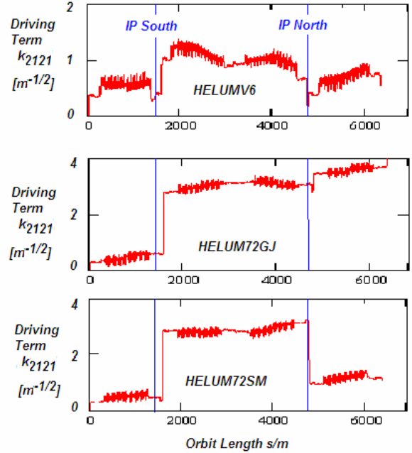
Figure 1: Build up of the driving term of the satellite resonance 2Q_x + Q_s = q around the circumference
