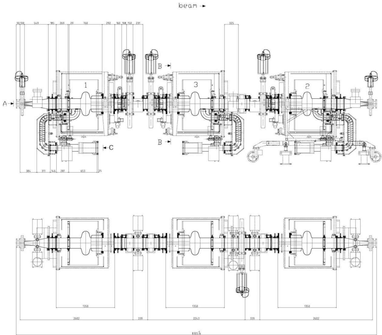
Figure 1: Layout of installation of three SRF 500 MHz accelerator modules in one straight of the Diamond Light Source. The total length for the installation is 8.3 m.
