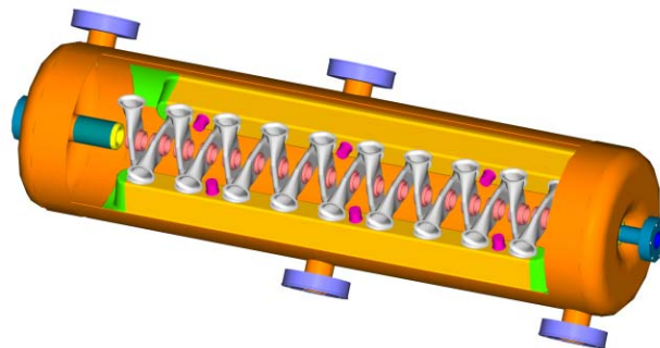
Figure 10: Cut view of the 352 MHz superconducting CH mode cavity.
