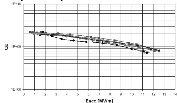
Figure 5: Summary of test results on 500 MHz single cell cavities of the Cornell design. All cavities show similar behaviour during RF test showing the reliable preparation procedure.
