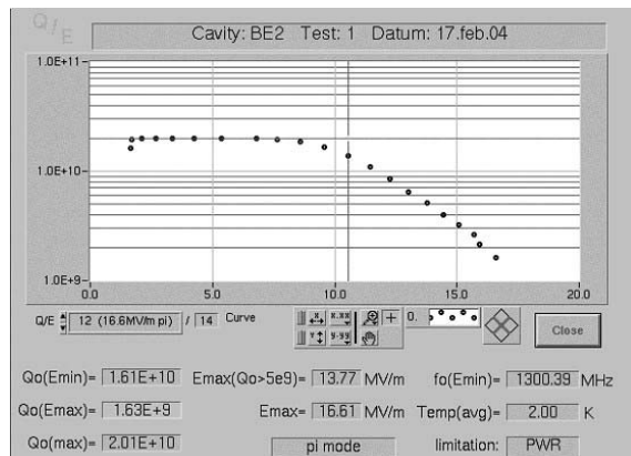
Figure 7: Test result of first prepared TESLA cavity BE1. Field emission was observed above 10 MV/m.
