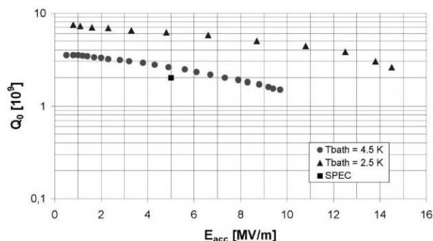
Figure 2: Typical result of a 400 MHz Nb/Cu plated cavity for LHC produced and prepared at ACCEL. The RF test was performed at CERN.
