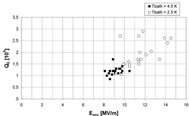
Figure 3: Highest gradients E_{acc} and quality factors Q_0 at the highest gradients achieved at bath temperatures of 4.5 K and 2.5 K in the 21 LHC 400 MHz single cell cavities. The tests were carried out at CERN.
