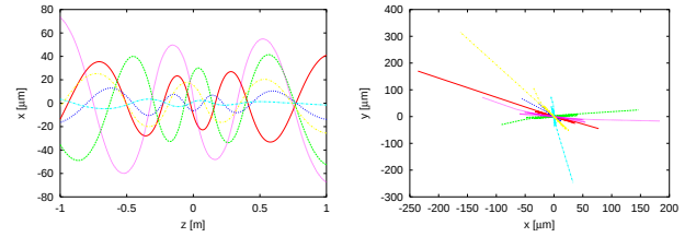
Figure 5: Simulated electron trajectories during the beam-beam collision. Left: Horizontal electron coordinate in microns as a function of the longitudinal position in m, for a 2-m long interaction region. Right: Projection of electron motion onto the x-y plane.
