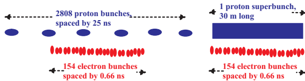
Figure 1: Bunch filling patterns in LHC and CLIC for the nominal LHC (left) and with an LHC superbunch (right).
