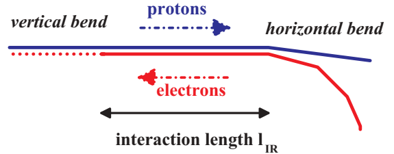
Figure 2: Schematic of IR layout, with horizontal and vertical dipoles for combining and separating the electron and proton beams.
