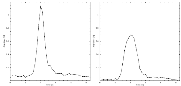
Figure 4: Typical low intensity bunches before ejection without (left) and with (right) phase noise for 3 s.
