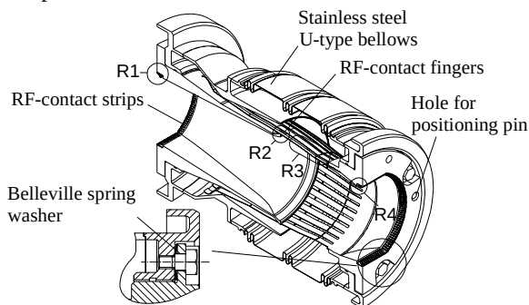
Figure 3 - Plug-in module.
