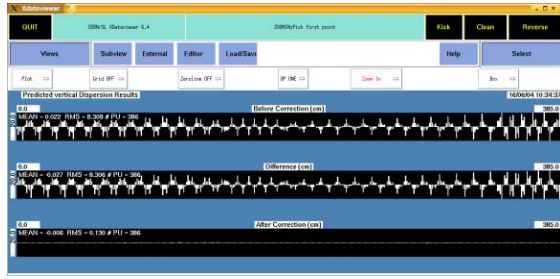
Figure 2: The dispersion correction of CLIC damping ring.
