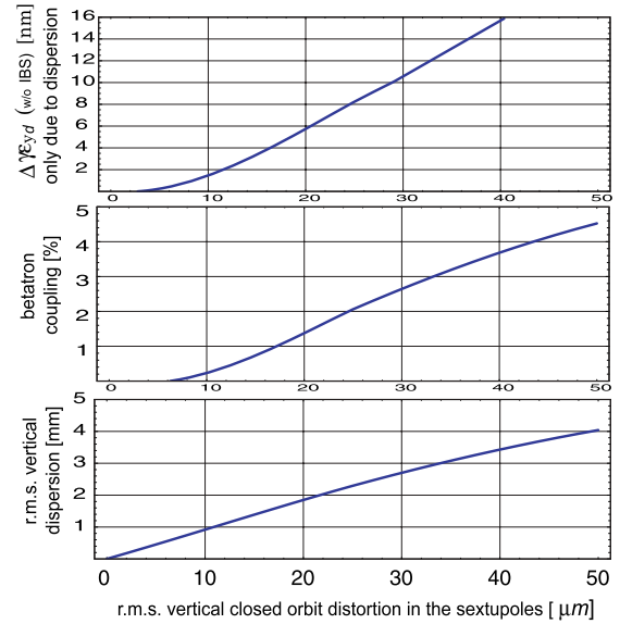
Figure 4: The dependance of betatron coupling, rms vertical dispersion and contribution to the vertical emittance due to vertical dispersion versus closed orbit distortion inside sextupoles.
