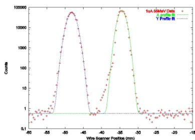
Figure 5: Beam profile after energy recovery for the 55MeV injection configuration.
