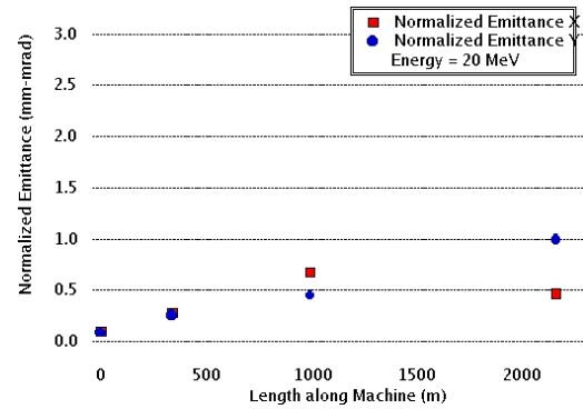
Figure 4: Emittance measurements for the 20MeV injector/dump energy.
