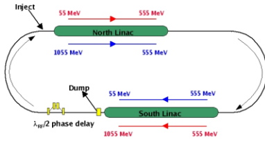
Figure 1: CEBAF Energy Recovery Experimental layout for the 55MeV injection configuration.
