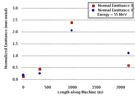
Figure 3: Emittance measurements for the 55MeV injector/dump energy.
