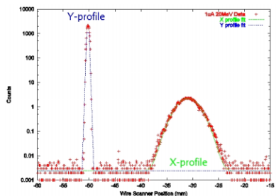
Figure 6: Beam profile after energy recovery for the 20MeV injection configuration.
