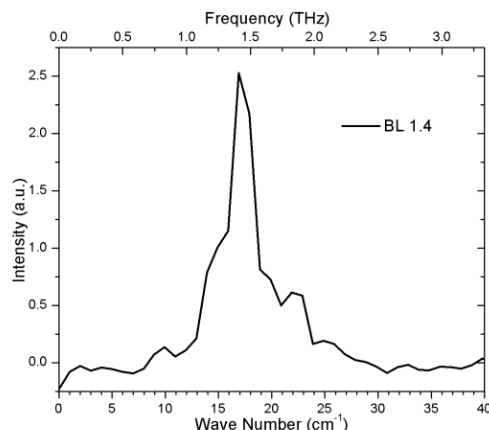
Figure 6: The spectral measurement of the infrared signal at BL1.4.
