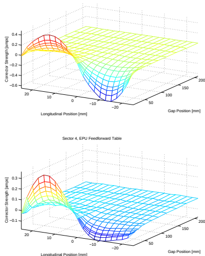
Figure 2: Two dimensional feed forward table used for orbit compensation of one of the EPUs (2 of the 4 correctors used are plotted).
