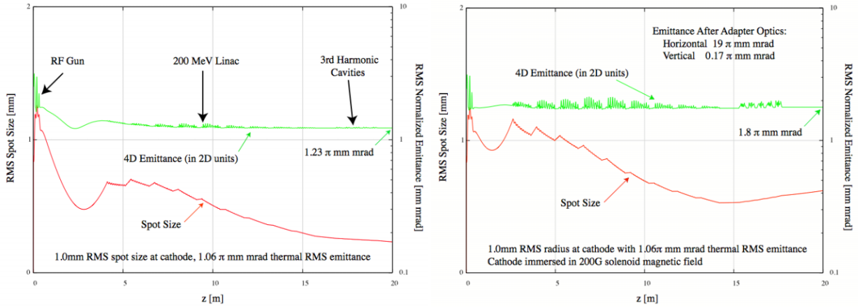
Figure 2. RMS emittance (2D) and spot size evolution ( \sigma_r ) from photocathode to the exit of the 3 rd harmonic cavities for ‘round’ beams (left) and ‘flat’ beams (right). The emittance is projected over the 35ps, 1nC beam core.
