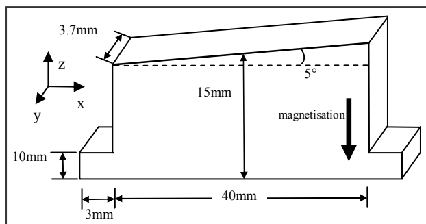
Figure 2: The dimensions of a canted magnet block.
