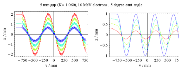
Figure 3: Electron trajectory through the undulator.
