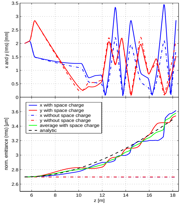
Figure 6: Transverse beam sizes and normalized emittance with and without space charge together with the analytic estimate for the second (long) transfer line.
