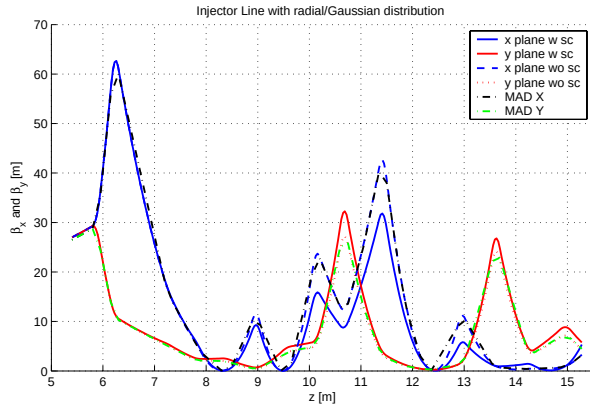
Figure 4: \beta function behaviour in the first (short) transfer line with and without space charge and original MAD matching.
