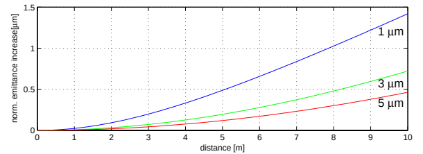
Figure 3: Emittance growth for 1 \mu\text{m} , 3 \mu\text{m} and 5 \mu\text{m} initial normalized emittances, 4 ps bunch length and 80 pC bunch charge.
