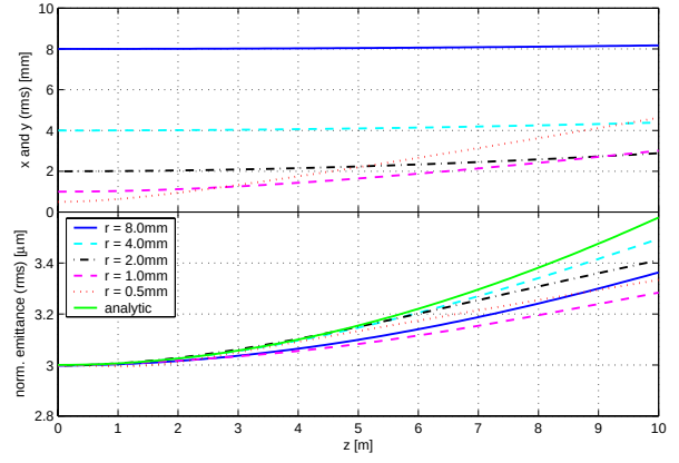
Figure 1: rms beam size and normalized emittance increase for \epsilon_0 = 3 \mu\text{m} , bunch length of 4 ps and charge of 80 pC.
