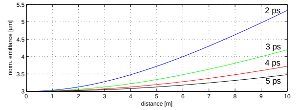
Figure 2: Emittance growth for 2 ps, 3 ps, 4 ps and 5 ps bunch lengths, 3 \mu\text{m} initial normalized emittance and 80 pC bunch charge.
