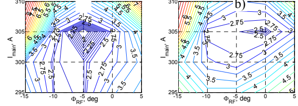
Figure 4: Contour plots of the measured horizontal (a) and vertical (b) normalized beam emittance [ \pi mm mrad] as a function of the RF phase and the main solenoid current.
