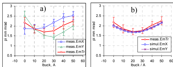
Figure 6: a) Measured transverse emittance as a function of bucking solenoid current. The RF phase is \Phi_0 - 5^\circ , the main solenoid current is 305 A. b) Simulated emittance as a function of the bucking solenoid current compared to measurements.
