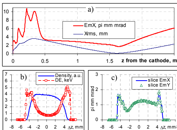
Figure 7: a) Simulated horizontal rms beam size and emittance along the beam line for the optimum parameter set. b) Bunch density distribution and slice energy spread for z = 1.62 m. c) Slice emittance distribution inside the bunch at z = 1.62 m.
