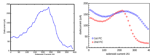
Figure 5: Darkcurrent of the RF gun measured with a pure molybdenum cathode inserted (without emissive film) at Faraday Cup 2 (left), and with the \text{Cs}_2\text{Te} cathode 42.2 after 80 days of operation at Faraday Cup 1 (right) (80 cm from the cathode – 1st FCup, blue) and 2 (130 cm from the cathode – 2nd FCup, red).
