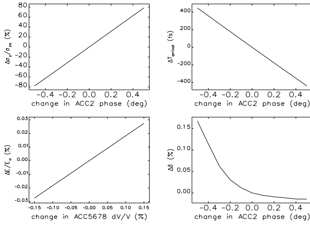
Figure 2: The most sensitive jitter source in rms bunch length (top left), bunch arriving time (top right), average beam energy (bottom left), and relative p2p energy deviation (bottom right).
