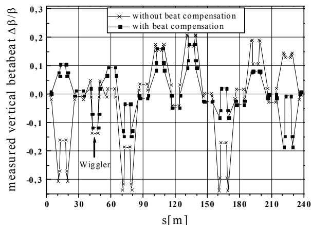
Fig. 6: Measurement of the vertical beta beat in the straight sections before and after compensation of the vertical optics
