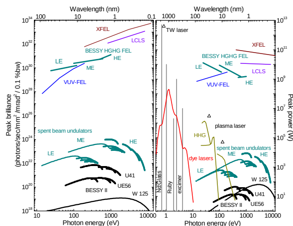
Figure 1: Peak brilliance and peak power from the BESSY-FEL compared to the BESSY II storage ring based light source, the DESY VUV-FEL, the European X-FEL and SLAC's LCLS.
