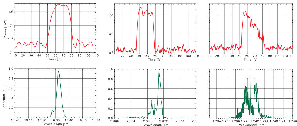
Figure 2: Simulation results for the cascaded BESSY HGHG-FEL-lines. Upper graphs time resolved power distributions, Lower graphs spectral power distributions. Data correspond to the high energy end of the 2 to 4 fold staged FEL-lines, corresponding to a wavelength of 10.3, 2.0 and 1.24 nm. In all cases a 17 fs (rms) Gaussian seed pulse of 500 MW peak power was assumed.
