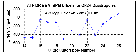
Figure 4: Offsets of BPMs with respect to centers of adjacent QF2 arc quadrupoles.
