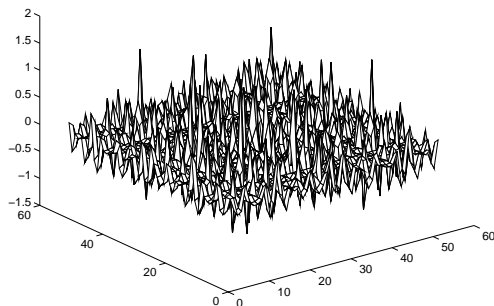
Figure 3: Chaotic-like behaviour.
