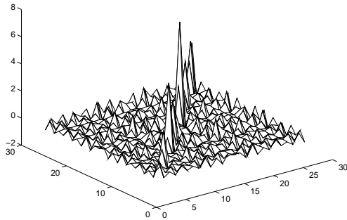
Figure 2: Stable wavelet pattern.
