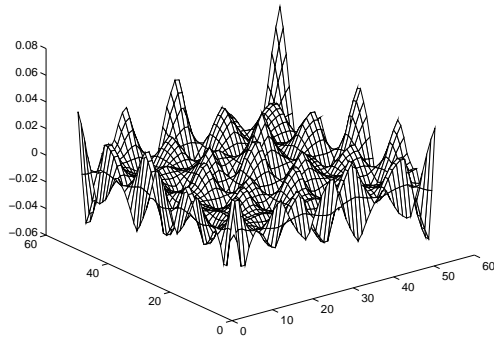
Figure 1: Eigenmode of level 1.
