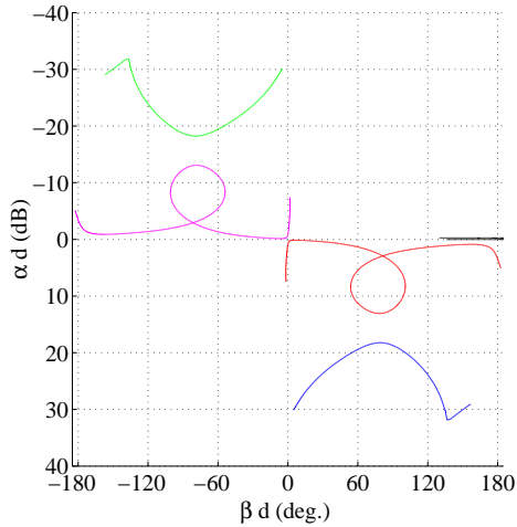
Figure 3: Speed-of-light line and projection in the (\beta d, \alpha d) plane of the dispersion diagram for the first two pairs of dipole modes
