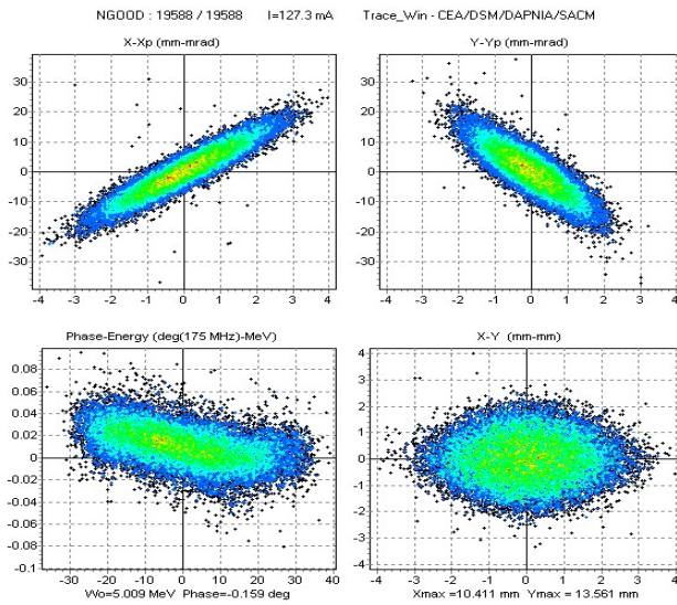
Figure 3: Beam distribution phase space at RFQ exit.
