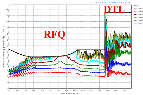
Figure 6: Beam size along the whole linac without errors
