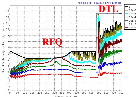
Figure 7: Beam size along the whole linac with full errors
