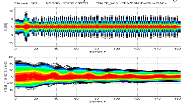
Figure 4: X and phase beam distribution along DTL.
