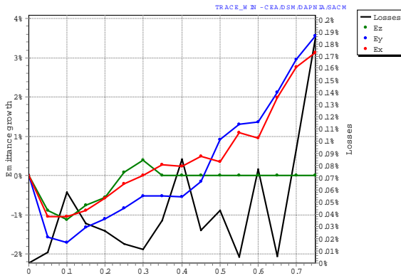
Figure 5: Emittances and losses growth in respect to machining defect (fraction of 100 \mu\text{m} ).
