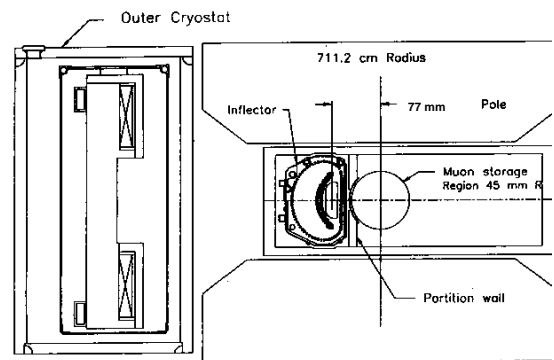
Figure 1: The inflector exit-vacuum chamber geometry. The center of the storage ring is to the right. The gap between the pole pieces is 180 mm, and the inflector exit is 18 \times 56 \text{ mm}^2 (ignoring the chamfer on the outer radius corners).
