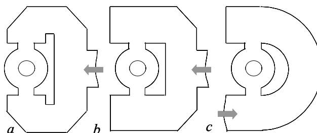
Figure 1. Three types of DFC couplers: a -standard [1], b - SBLC DESY, [2], c - J-type, JLC, KEK [4].
