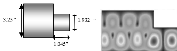
Figure 2: TE_{01} - TE_{02} reflective mode converter. The dimensions shown are for an operating frequency of 11.424 GHz. The field pattern shown from finite element simulations predicts a peak electric field of 26.6 MV/m for 300 MW of input power.
