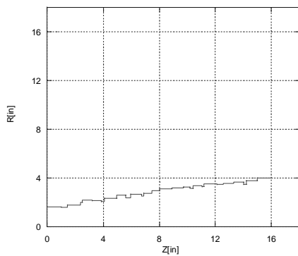
Figure 5a: End taper design for a 4-mode system. The plot shows the radius versus the axial distance of taper.
