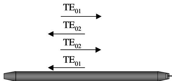
Figure 1: Dual-Moded Delay Line
