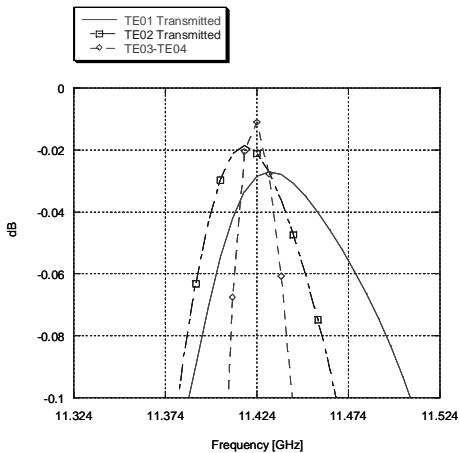
Figure 5b: Simulated response of input taper for a 4-mode system
