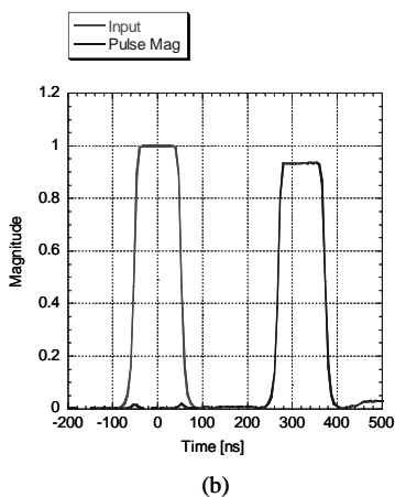
Figure 3: (a) Measured delay through 75 feet of WC475 waveguide terminated with a flat plate. The round trip delay time is 154 ns. (b) Measured delay through 75 feet of WC475 waveguide terminated with the TE_{01} - TE_{02} mode converter. The round trip delay time is 320 ns. The operating frequency is 11.424 GHz.
