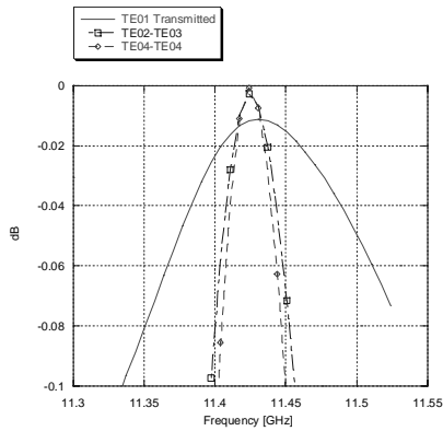
Figure 4:b: Simulated response of input taper for a 4-mode system
