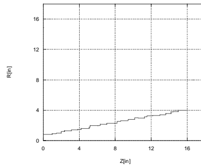
Figure 4a: Input taper design for a 4-mode system. The plot shows the radius versus the axial distance of taper
