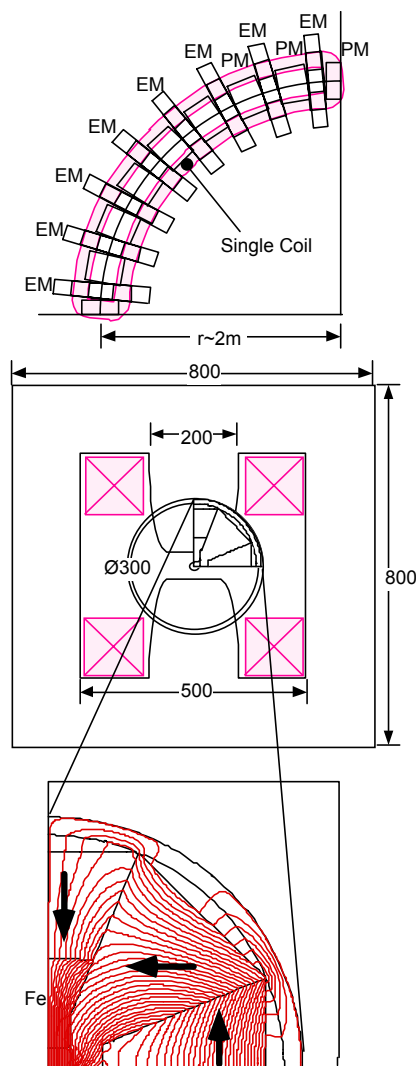
Figure 3. Longitudinal Magnet-in-Magnet (bird view). EM: Electro magnet. PM: permanent magnet.
