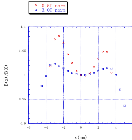
Figure 6. Field distribution at 0.5 Tesla and 3 Tesla.
