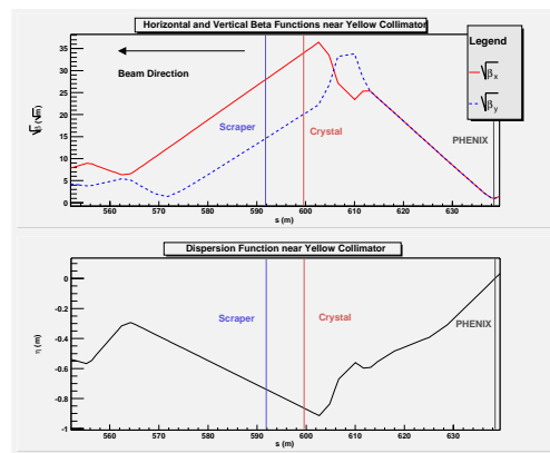
Figure 3: Beta function (top) and dispersion (bottom) in the yellow ring close to the collimators.
