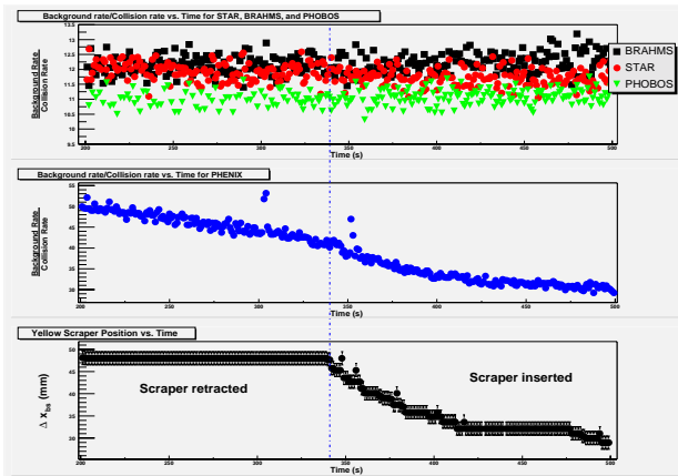
Figure 5: Background as a function of scraper position during Au operation. \beta^* = 2 m at all IRs.
