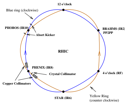
Figure 1: Location of the collimators and experiments in the RHIC rings.
