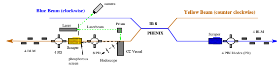
Figure 2: The RHIC collimation system
