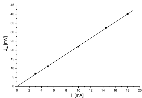
Figure 1: Dependency of the radiation-acoustic signal amplitude U_m from the beam current I_p .
