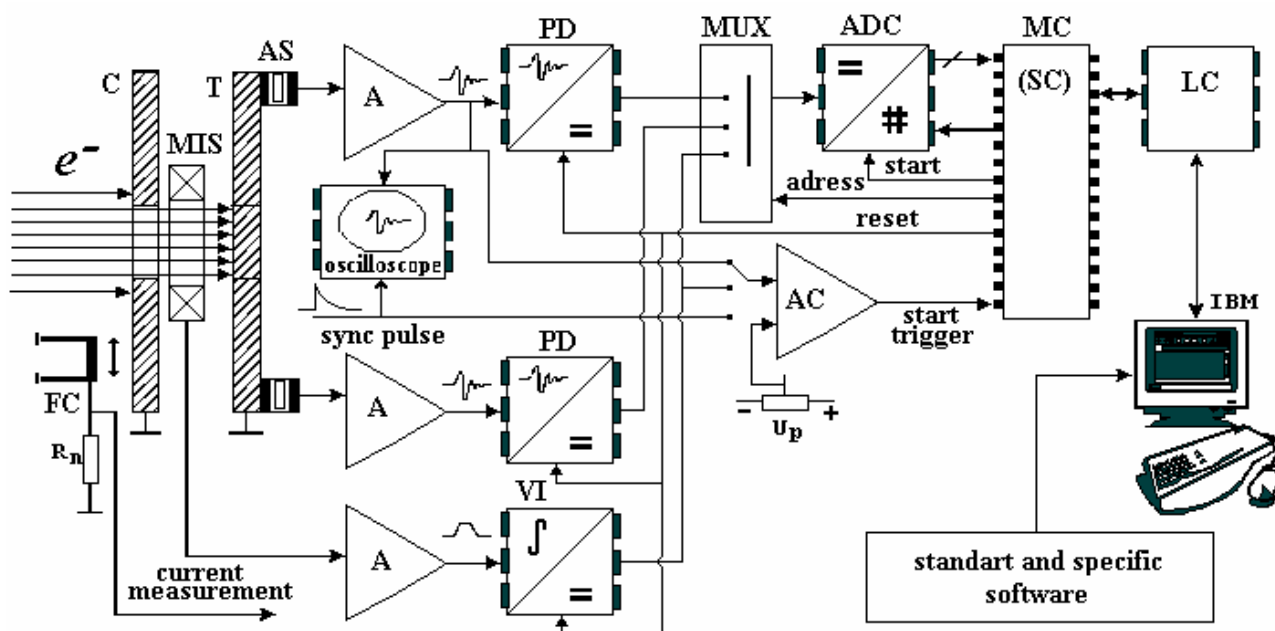
Figure 3: Scheme of experimental plant
