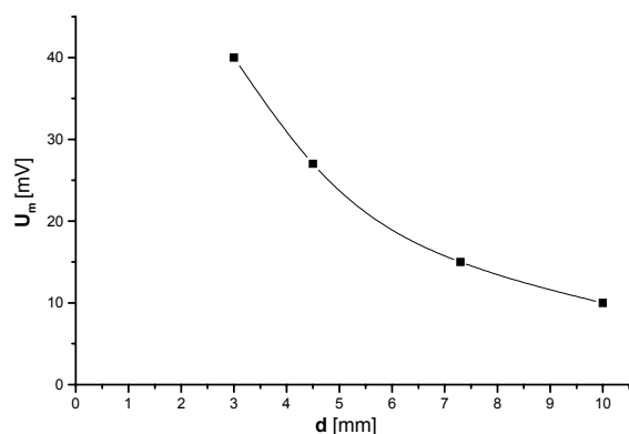
Figure 2: Dependency of the radiation-acoustic signal amplitude U_m from the beam's diameter d .
