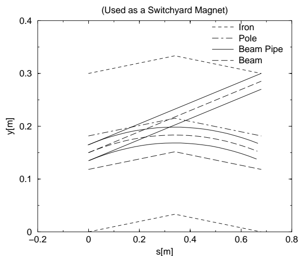
Figure 3: the trajectories and beam pipes of the switch yard magnet within the iron of the synchrotron dipole
